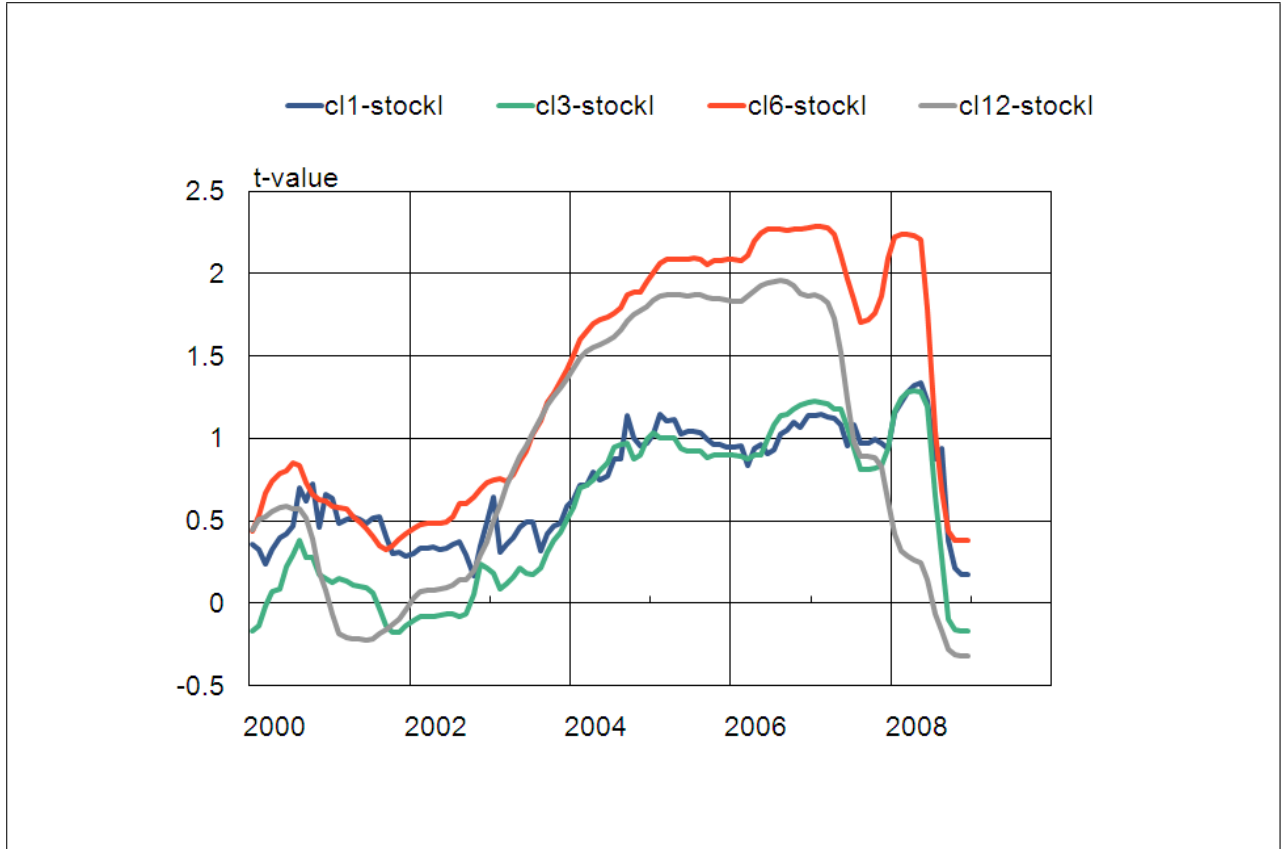
T-statistics in the rolling risk premia regressions for stockl
