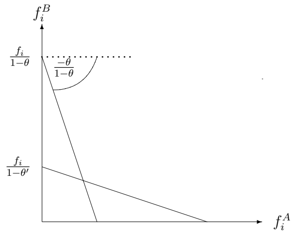
Figure 9: Broker i investors' fee settings, f_i^A and f_i^B , given the broker's fee, f_i . The two cases drawn satisfy 0 < \theta' < 1/2 < \theta < 1 .
