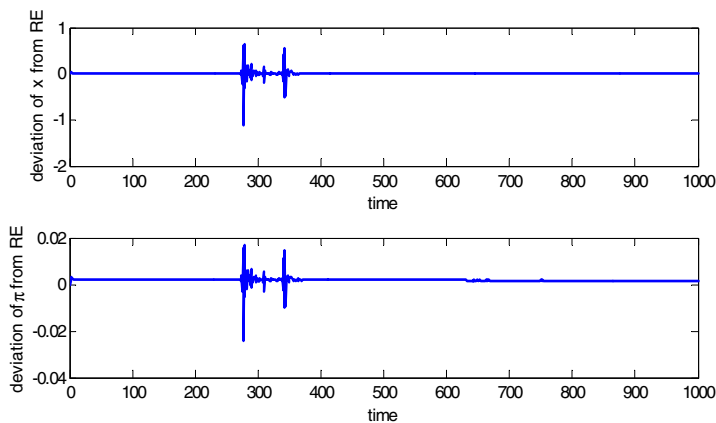
Figure 3.1 Stability of optimal Taylor-type rule with \gamma = 0.02 .
