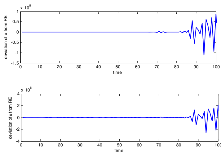
Figure 3.2 Instability of optimal Taylor-type rule with \gamma = 0.04 .
