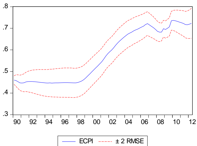
Smoothed ECPI State Estimate
