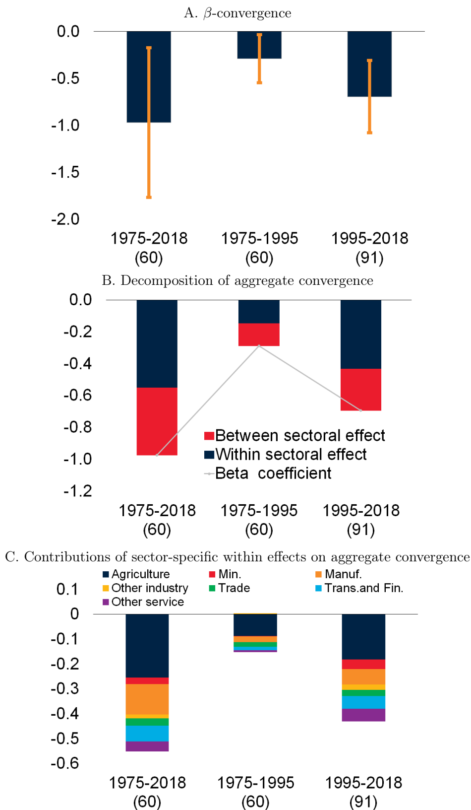
Figure 5: Decomposition of \beta -convergence
