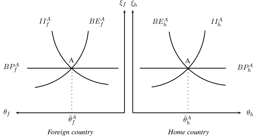
Figure 3: World initial equilibrium
