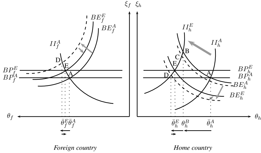
Figure 4: World effect of a domestic liquidity supply shock
