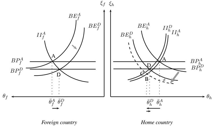
Figure 5: World effect of a domestic rise in bank fund-raising costs
